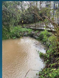
Downstream culvert outlet submerged, tidal backwater
