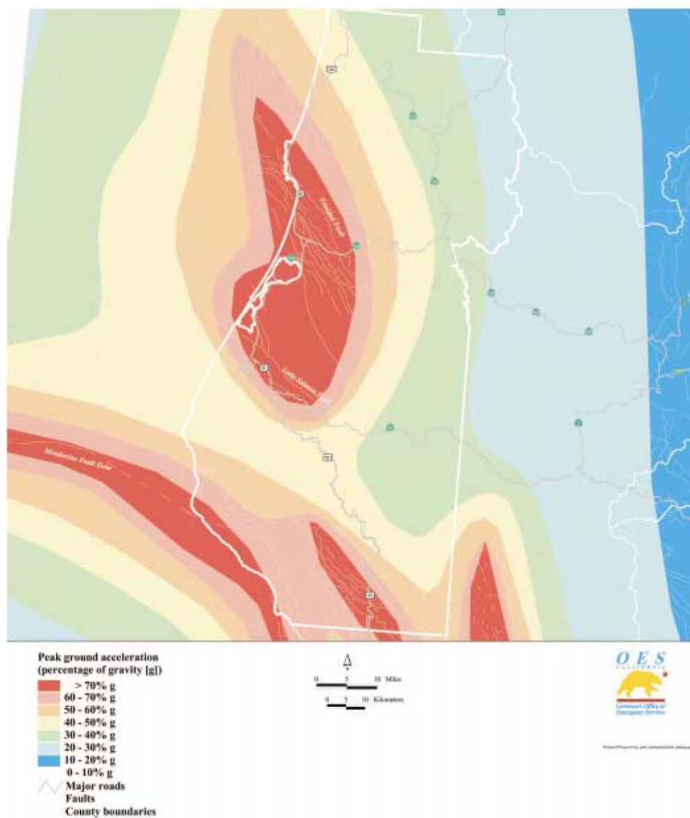
Figure 10-2 Probabilistic Ground Shaking, 10% Probability of Being Exceeded in 50 Years
